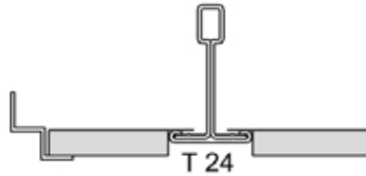
Tegular Lay-In Sistem
