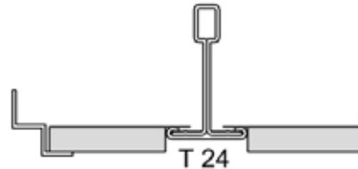
Tegular Lay-In Sistem
